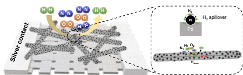
Schematic illustration of the hydrogen sensor based upon platinum-decorated palladium nanowires
